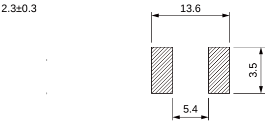
Land Pattern: [mm]
